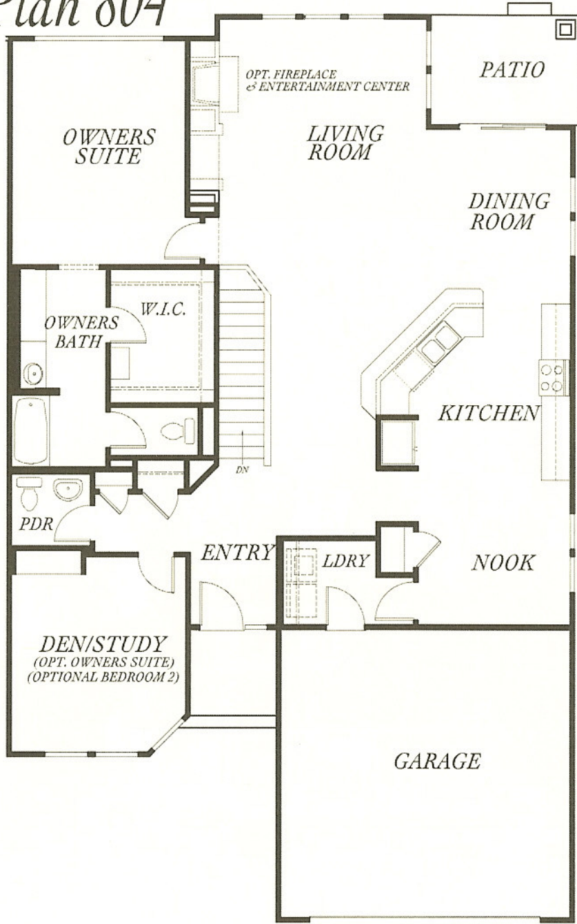
804 BASE PLAN
